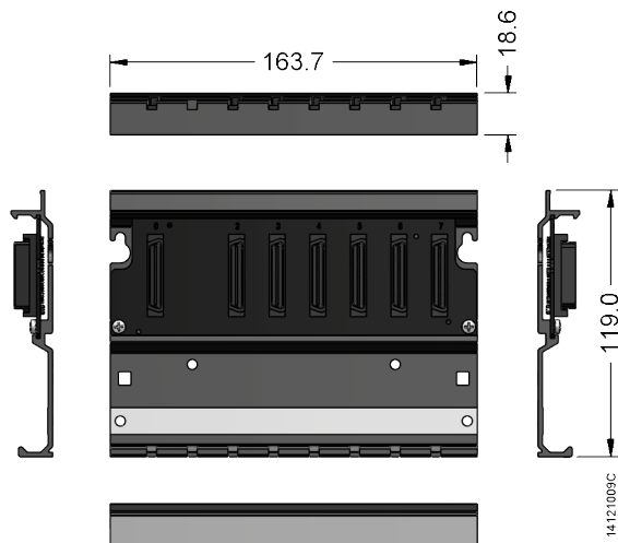
Figure 21: 8-Slot Backplane Rack (Without Hot Swap)
