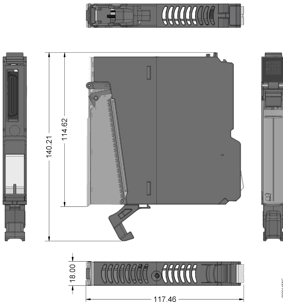
Figure 16: Nexto 18mm I/O Module
