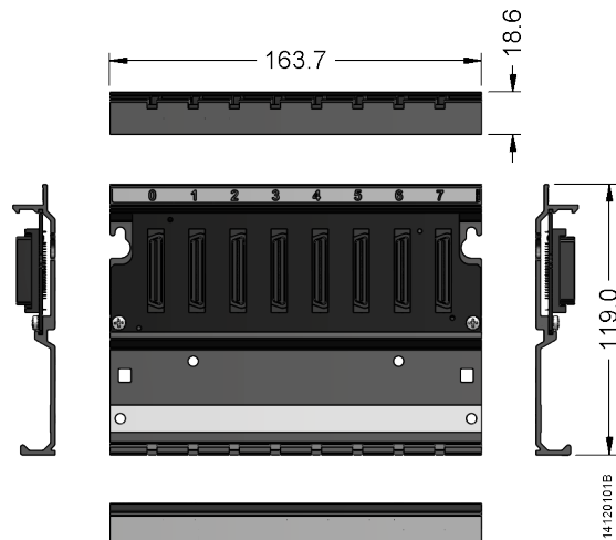
Figure 22: 8-Slot Backplane Rack
