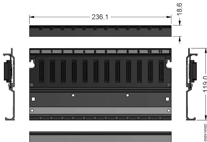
Figure 23: 12-Slot Backplane Rack
