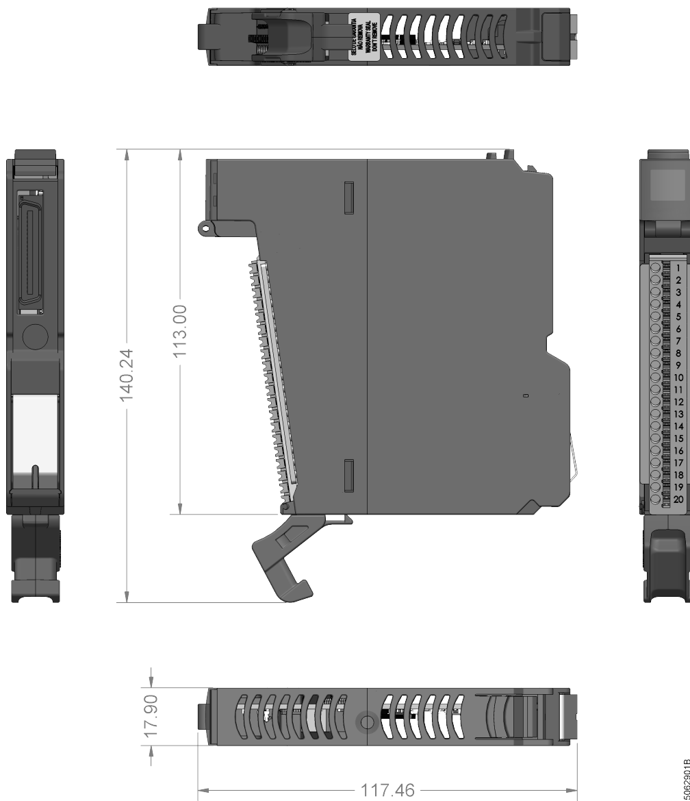
Figure 17: Nexto Jet 18mm I/O Module
