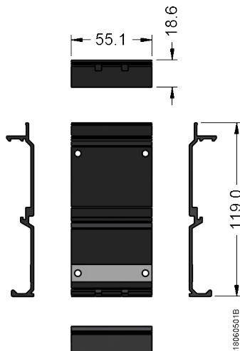
Figure 20: 2-Slot base for panel assembly
