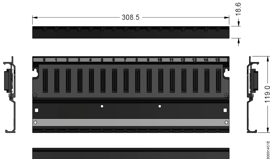
Figure 24: 16-Slot Backplane Rack
