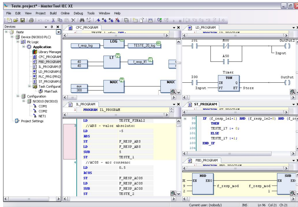
Figure 26: IEC 61131-3 Programming Languages
