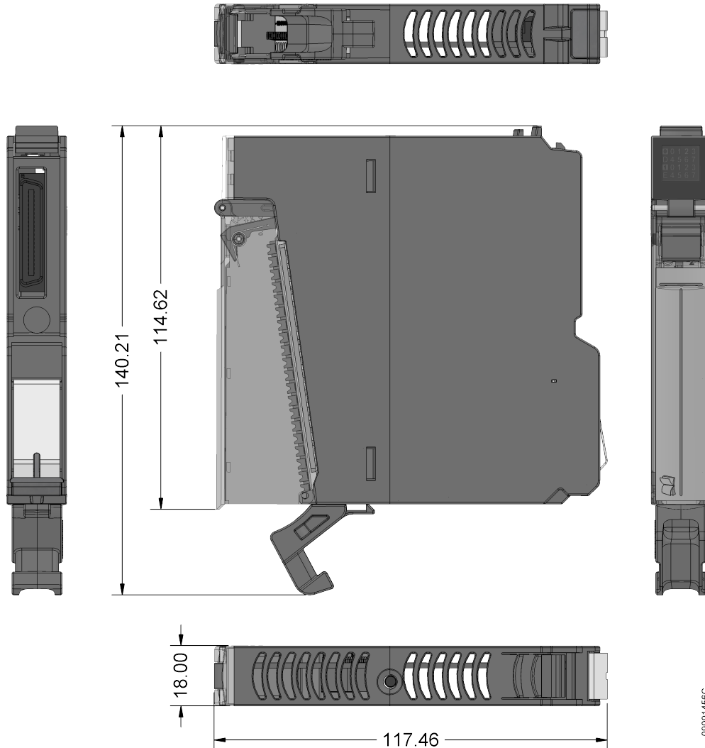
Figure 3: Physical Dimensions
