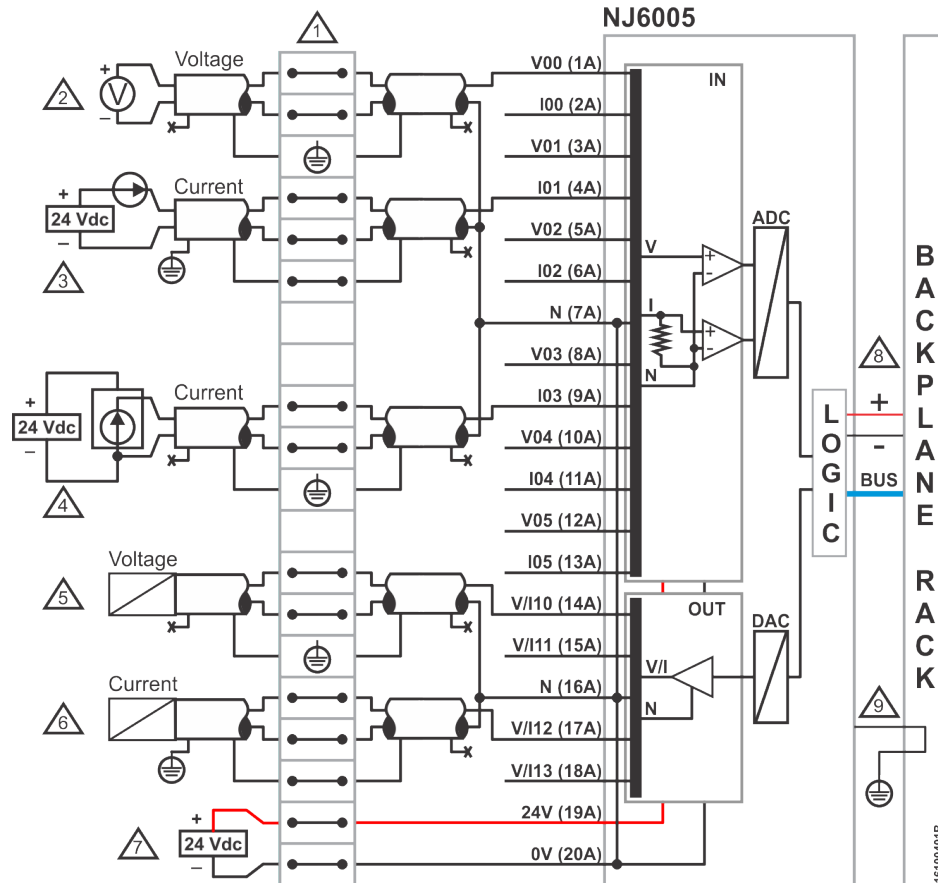
Figure 2: Electric Diagram
