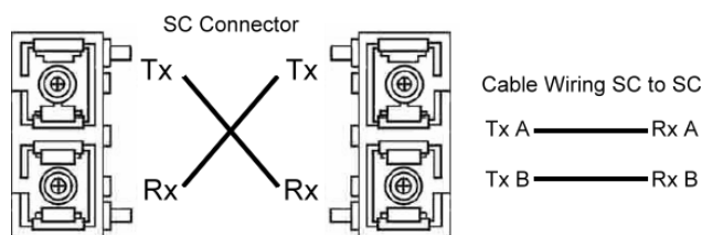
Figure 22: SC Multimode Connector Fiber Port
