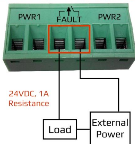
Figure 31: Connecting the Fault Alarm Contact for ET5-0500, ET5-0600, ET5-0602-M, ET5-0802-M, ET5-0800 E ET5 1204-SFP switches.
