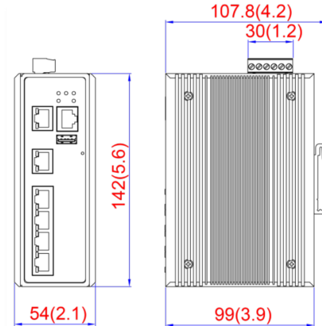
Figure 4: ET5-0600 Physical Dimensions
