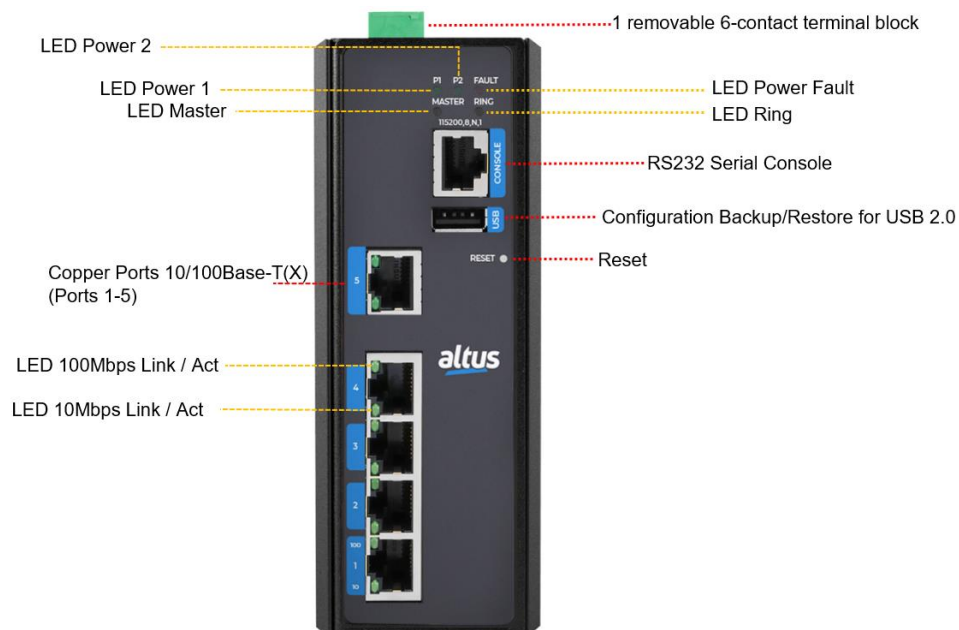
Figure 2: ET5-0500 Front Panel
