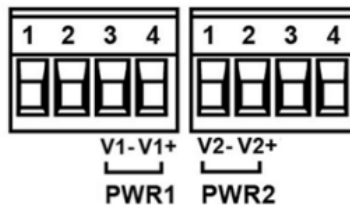
Figure 29: Power Terminal Block
