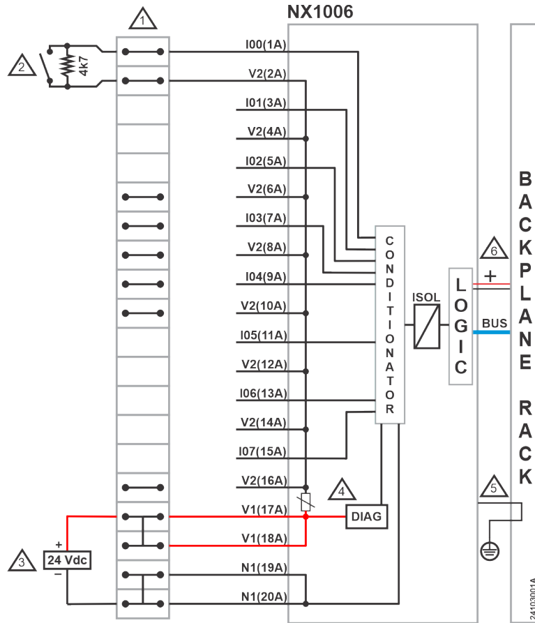
Figure 3: Electric Diagram
