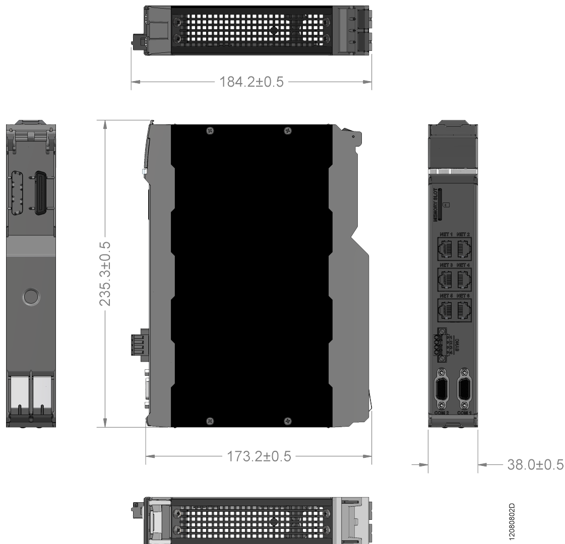
Figure 2: Physical Dimensions
