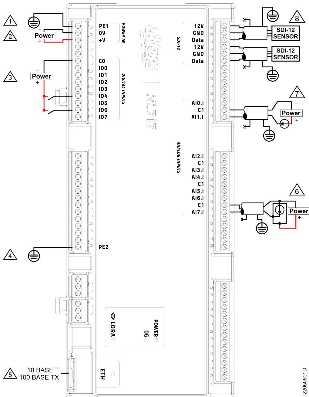
Figure 1: Electrical Installation
