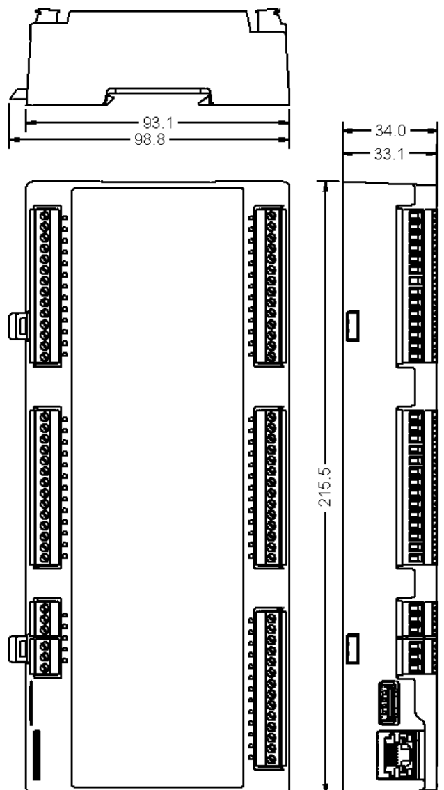
Figure 2: Physical Dimensions
