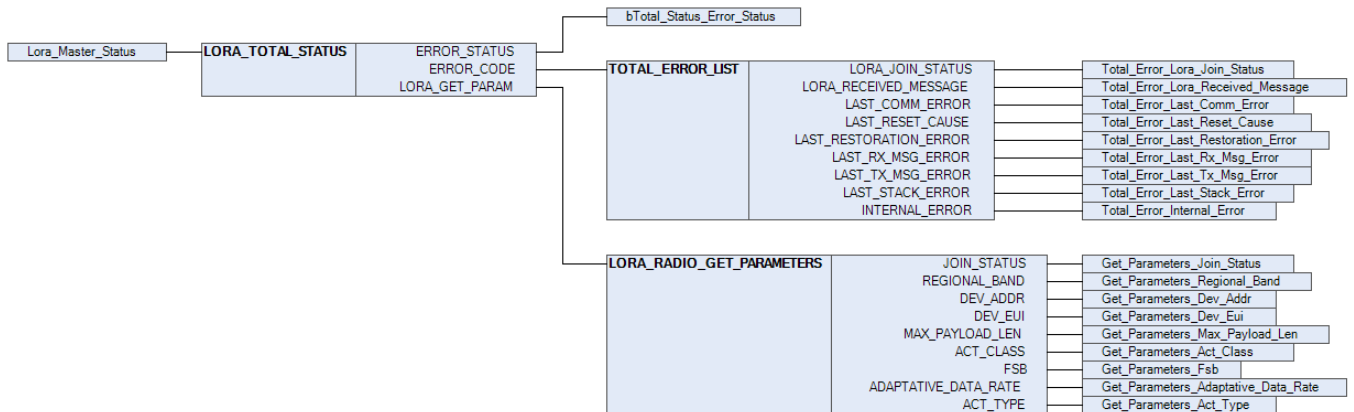
Figura 15: LORA_TOTAL_STATUS
