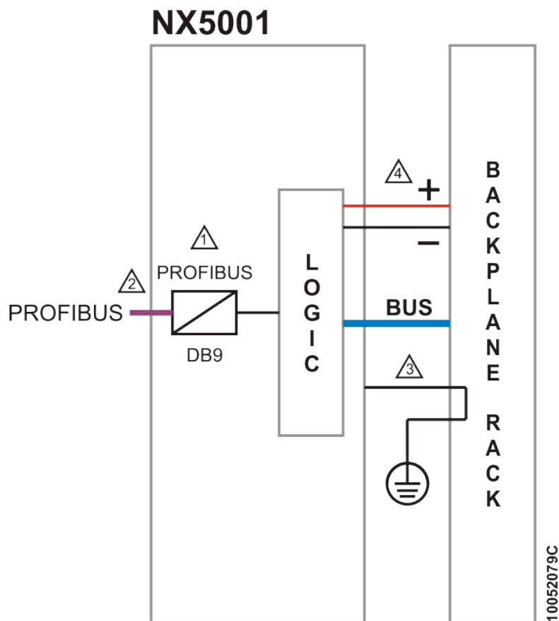
Figure 8: Electrical Diagram from NX5001
