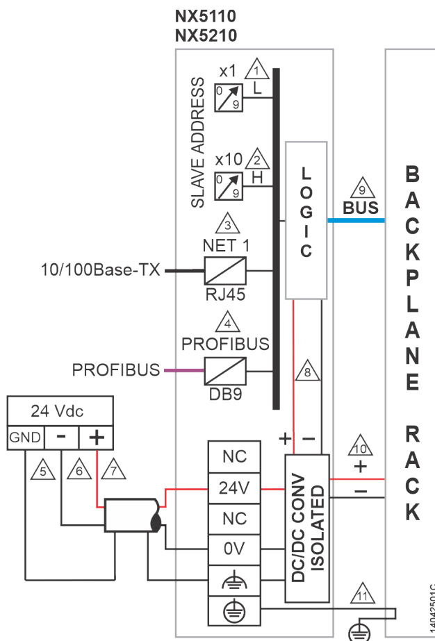
Figure 6: Electrical Diagram
