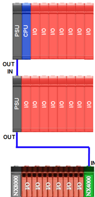
Figure 12: Bus Expansion with Xtorm and Nexto
