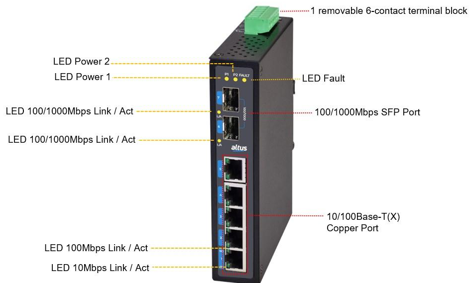
Figure 14: ET2-0702-SFP Front Panel
