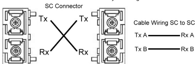
Figure 19: SC Multimode Connector Fiber Port
