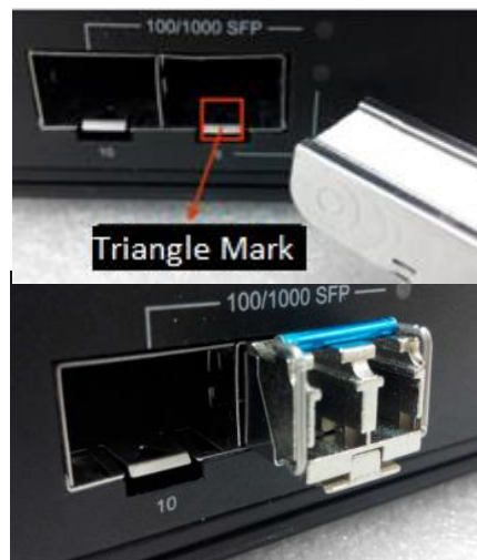
Figure 21: Transceiver inserted
