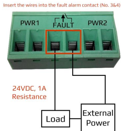
Figure 29: Connecting the Fault Alarm Contact for ET2-0800, ET2-0602-M, ET2-1600, ET2-0702-SFP and PT2-0500-24 switches.
