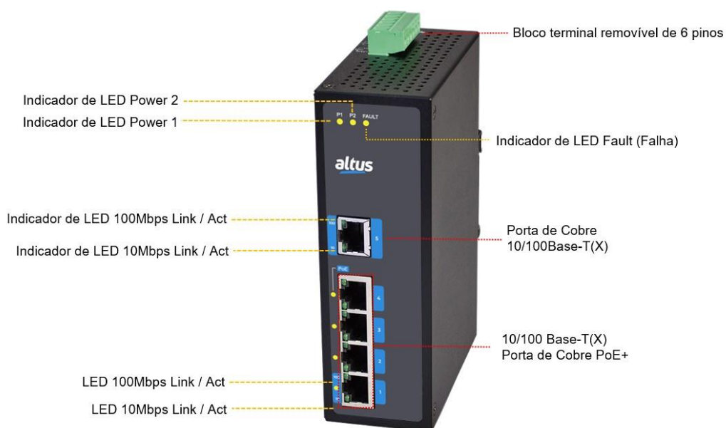
Figura 17: Painel Frontal do PT2-0500-24
