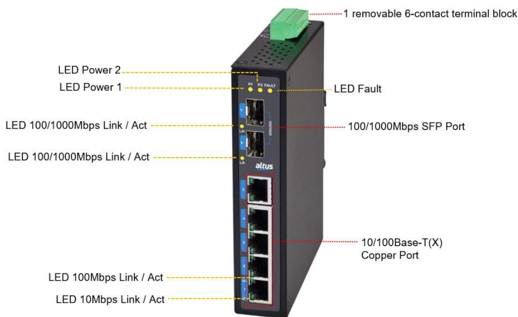
Figura 14: Painel Frontal do ET2-0702-SFP
