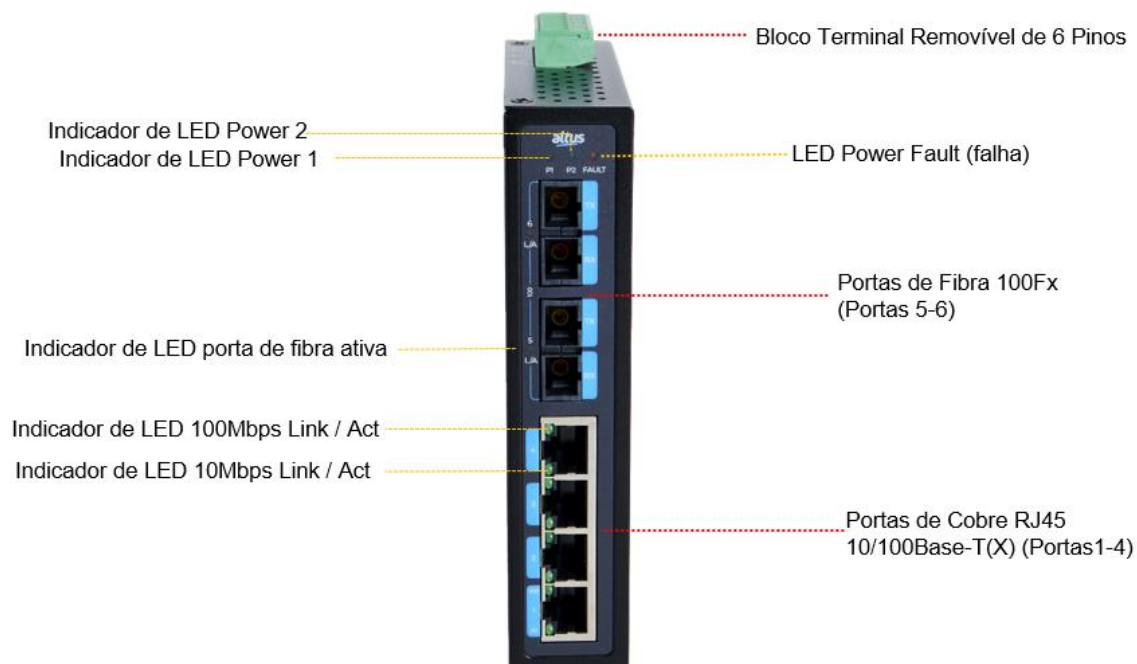
Figura 8: Painel Frontal do ET2-0602-M
