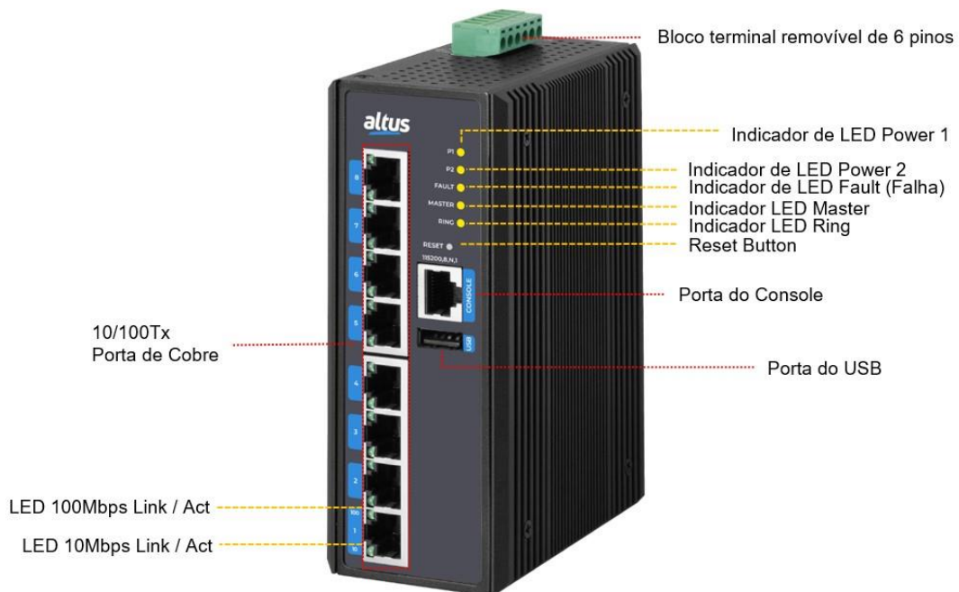
Figura 14: Painel Frontal do ET5-0800
