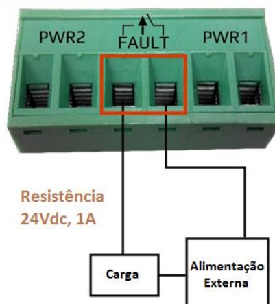
Figura 31: Conectando o Contato de Alarme Fault nos Switches ET5-0500, ET5-0600, ET5-0602-M, ET5-0802-M, ET5-0800 E ET5 1204-SFP.
