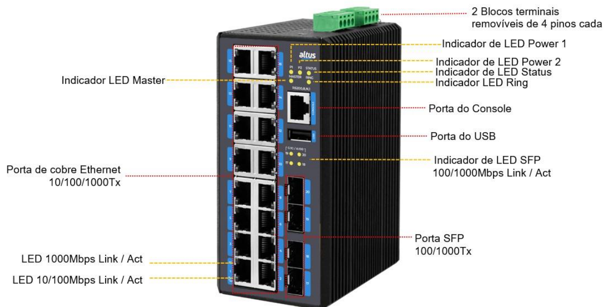
Figura 20: Painel Frontal do EG5-2004-SFP
