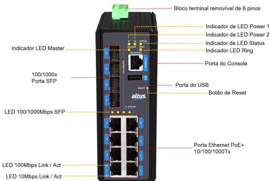
Figura 17: Painel Frontal do PG5-1204-SFP
