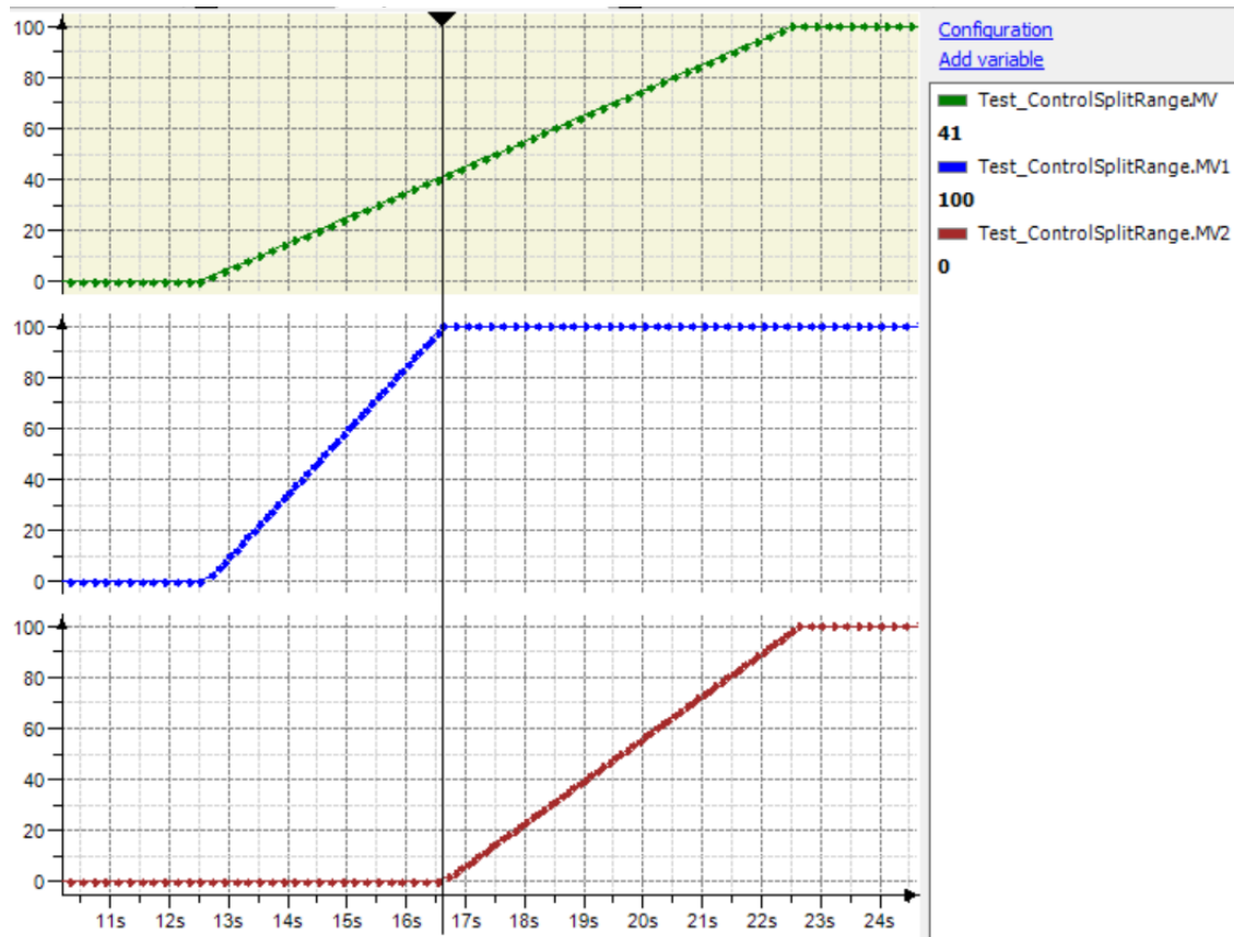
Figure 42: ControlSplitRange with Mode = 2 and SPLIT = 40%
