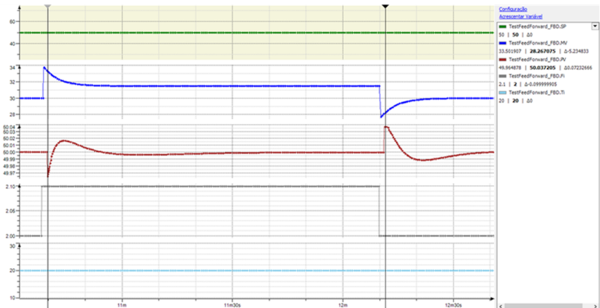
Figure 63: Effect of disturbances in Fi with feed-forward
