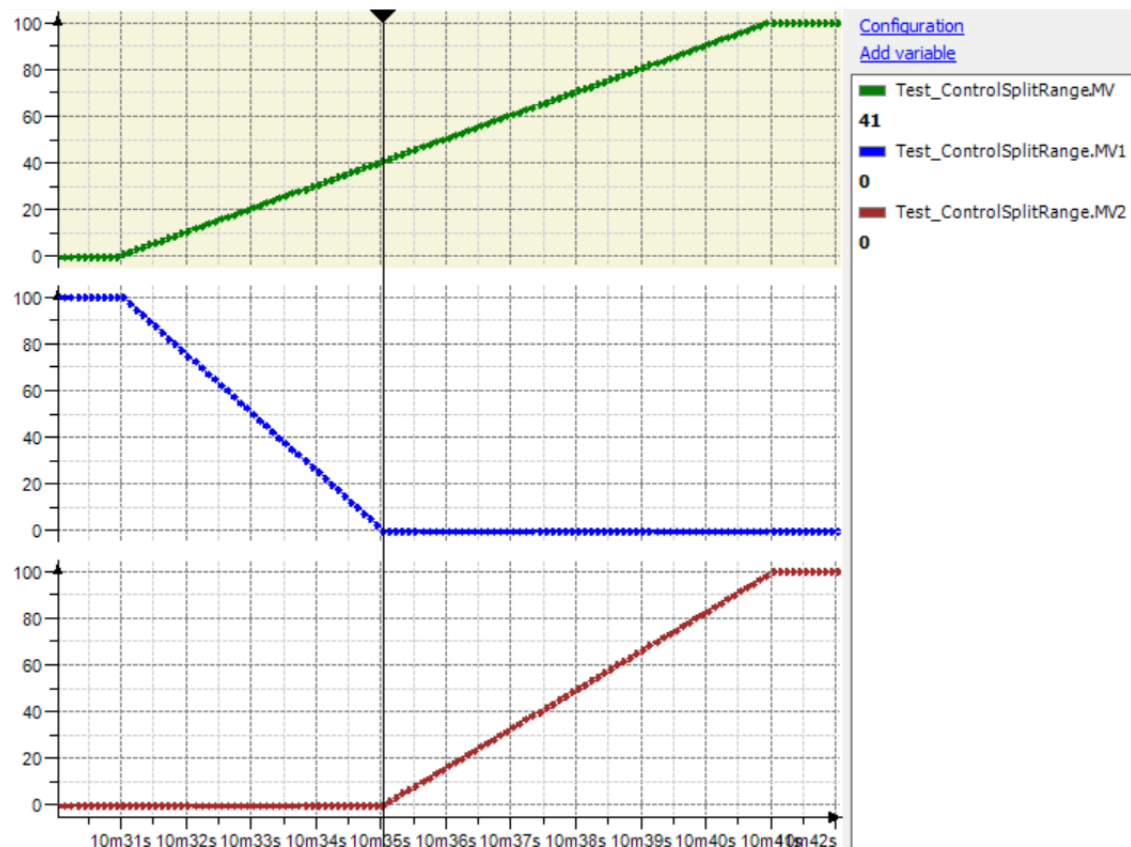
Figure 44: ControlSplitRange with Mode = 4 and SPLIT = 40%
