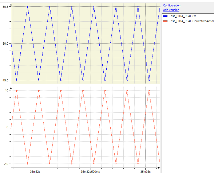
Figure 4: Effect of noise in derivative response with T_{fd} = 0 seconds
