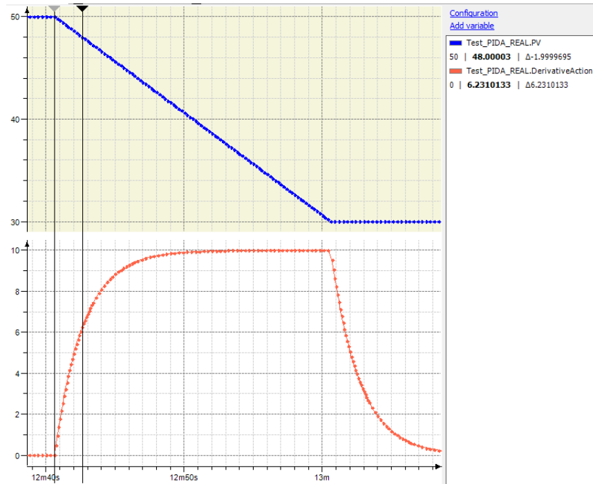
Figure 3: Derivative response with T_{fd} = 2 seconds
