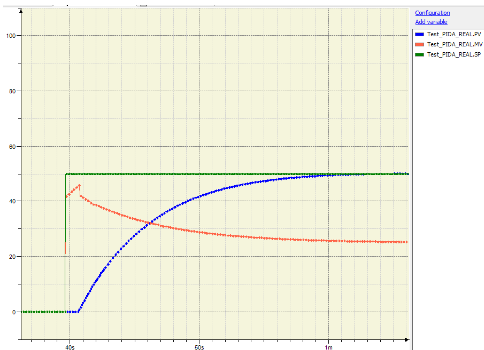
Figure 6: Response with MaxVarMV = 0 (no limitation, faster)
