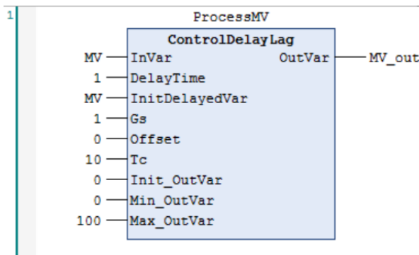
Figure 52: Network 1 of feed-forward example
