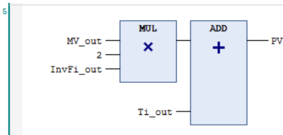
Figure 56: Network 5 of feed-forward example
