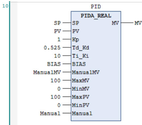
Figure 61: Network 10 of feed-forward example
