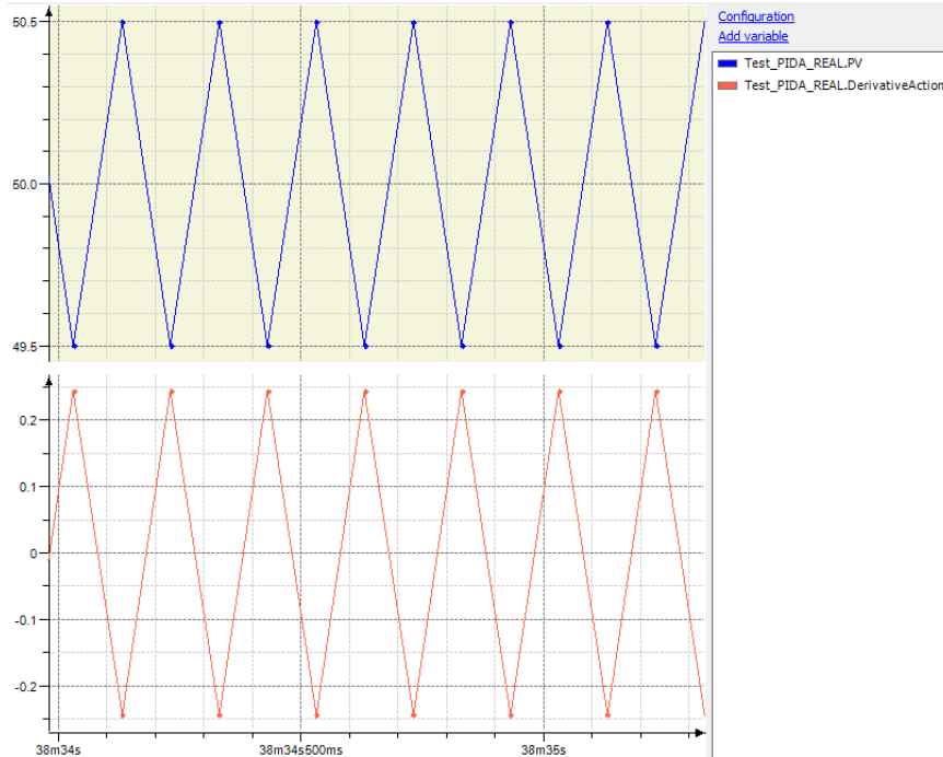
Figure 5: Effect of noise in derivative response with T_{fd} = 2 seconds
