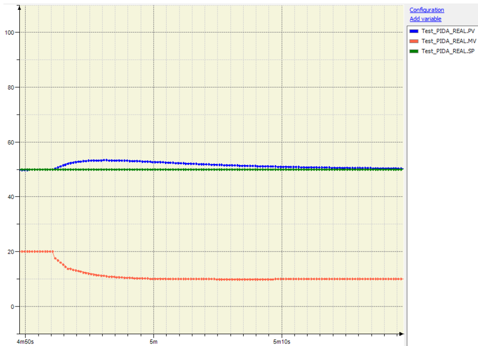
Figure 9: Example with reverse control (Direct = FALSE)
