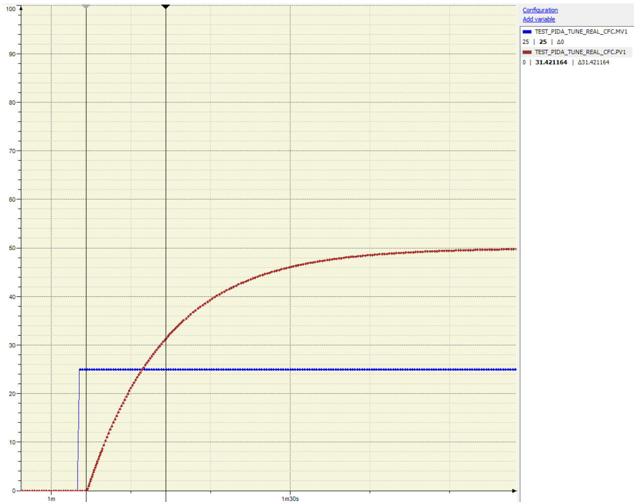
Figure 68: Open-loop characterization of process - time constant
