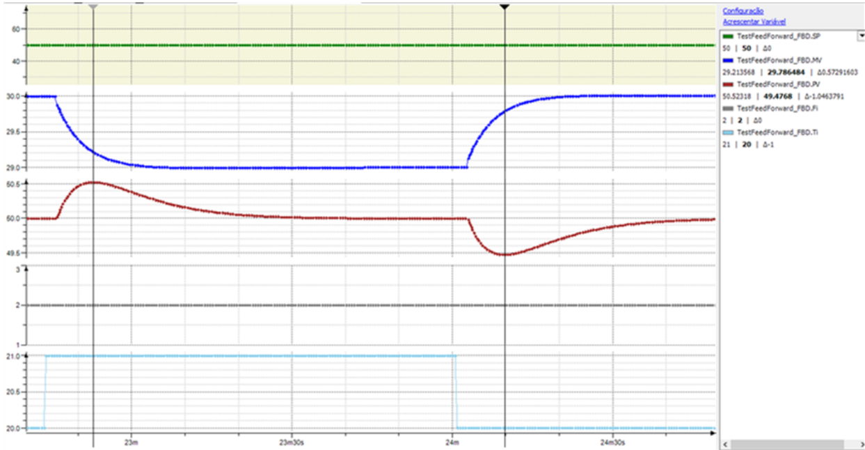
Figure 64: Effect of disturbances in Ti without feed-forward
