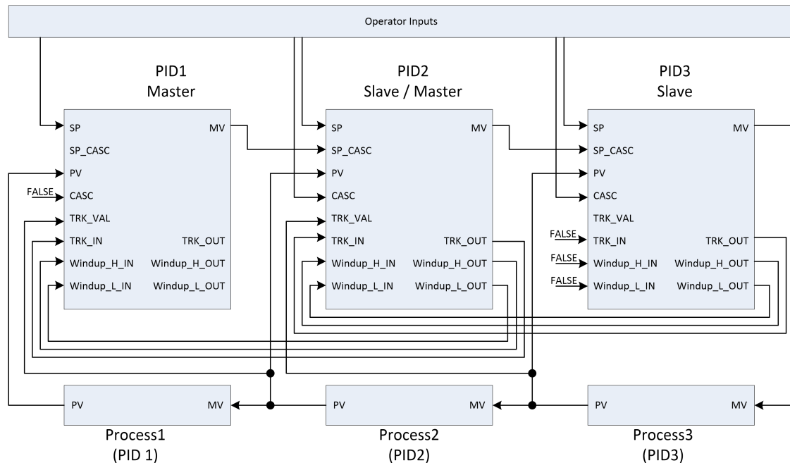
Figure 48: Special connection in cascade configurations
