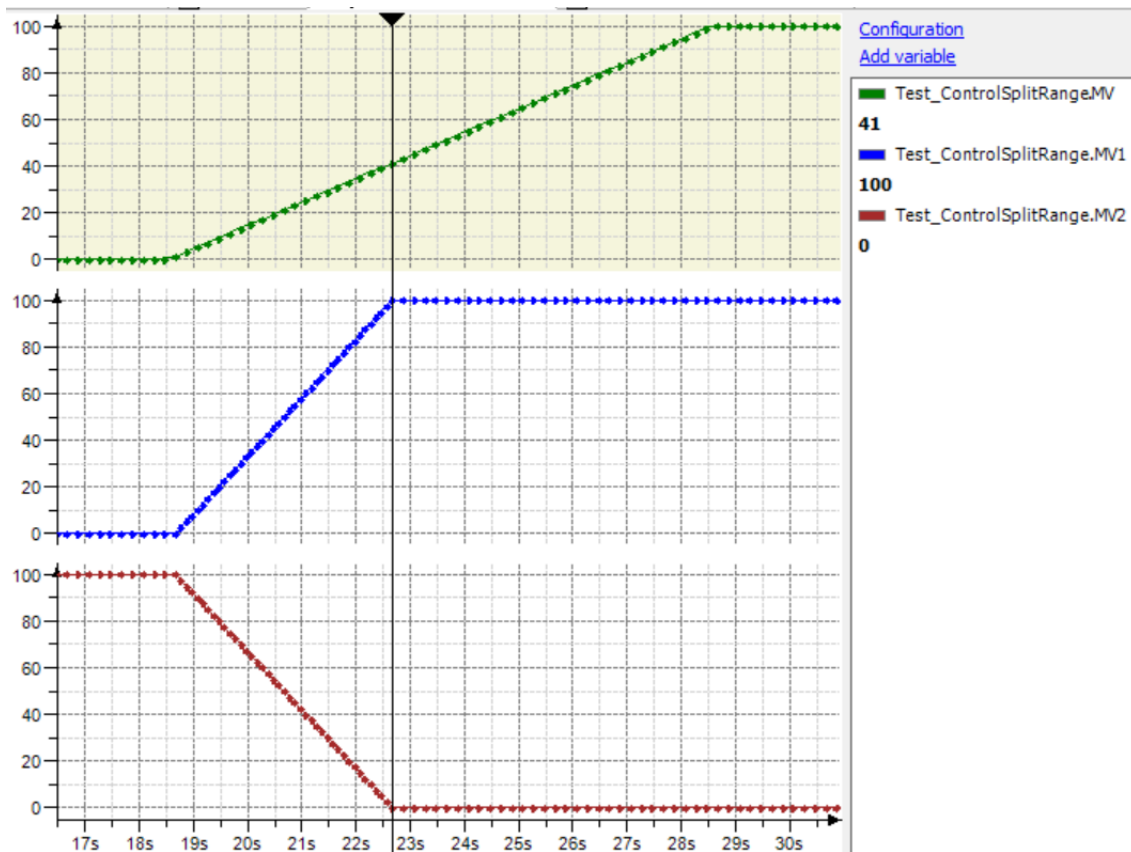
Figure 41: ControlSplitRange with Mode = 1 and SPLIT = 40%
