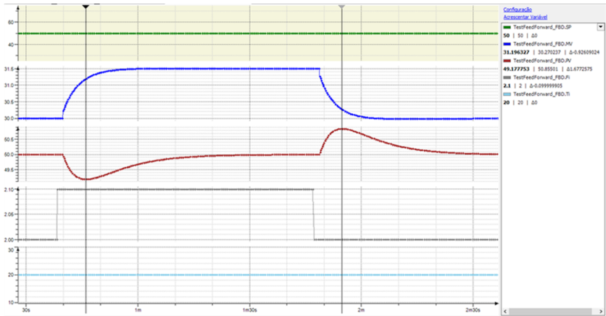
Figure 62: Effect of disturbances in Fi without feed-forward
