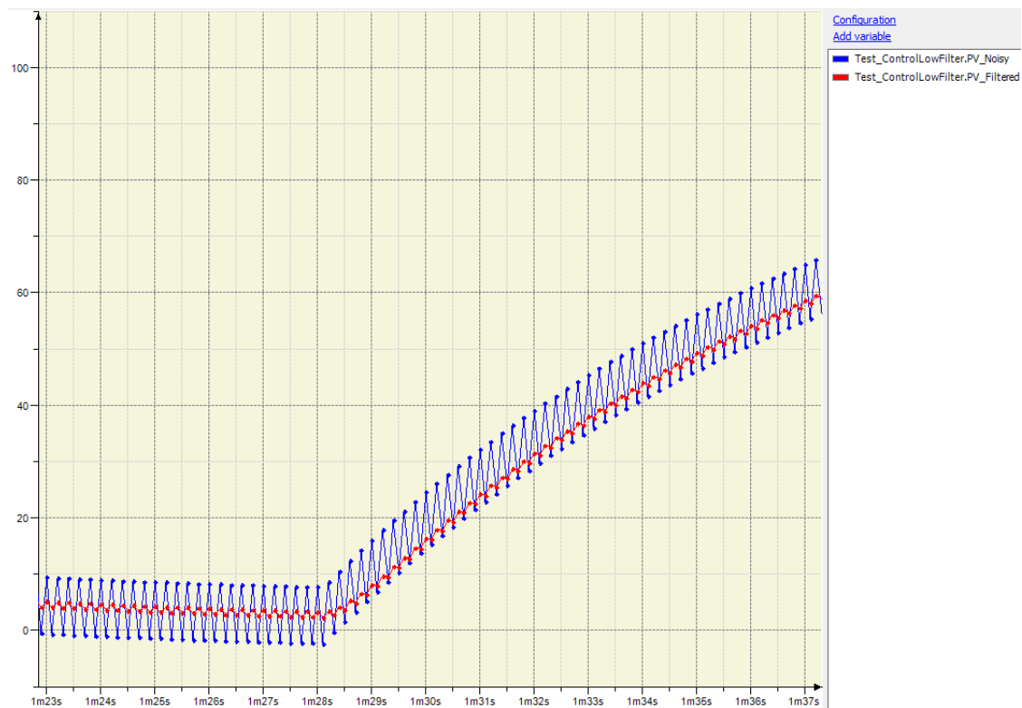
Figure 27: Example of filtering with ControlLowFilter
