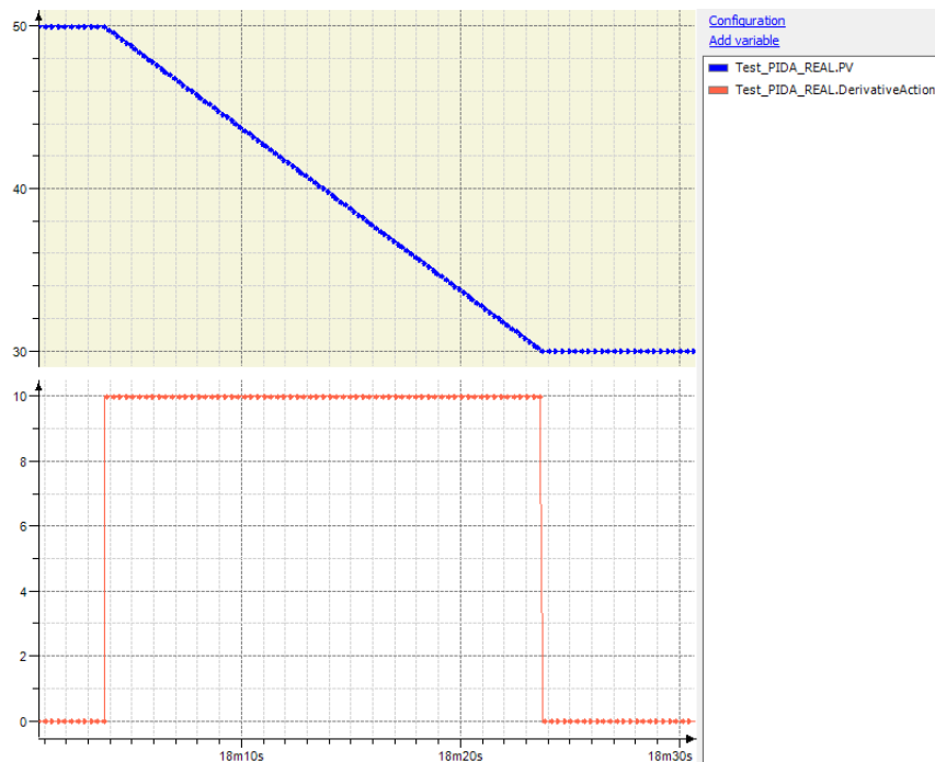
Figure 2: Derivative kick with Tfd = 0 seconds
