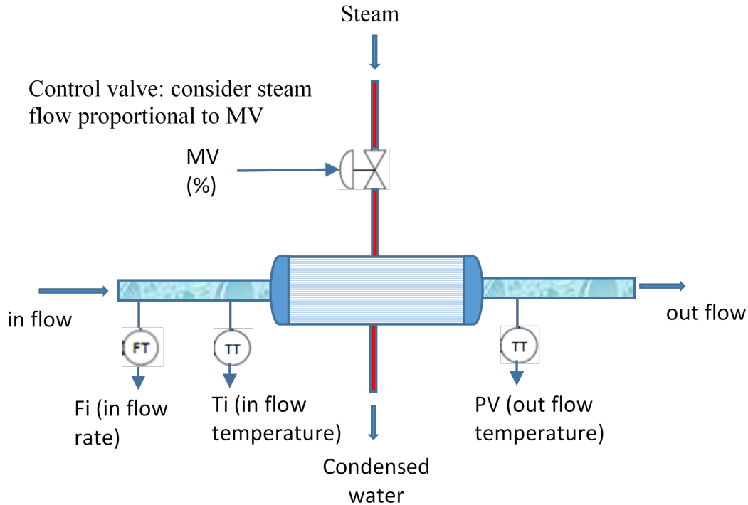
Figure 51: Simulated process for feed-forward control
