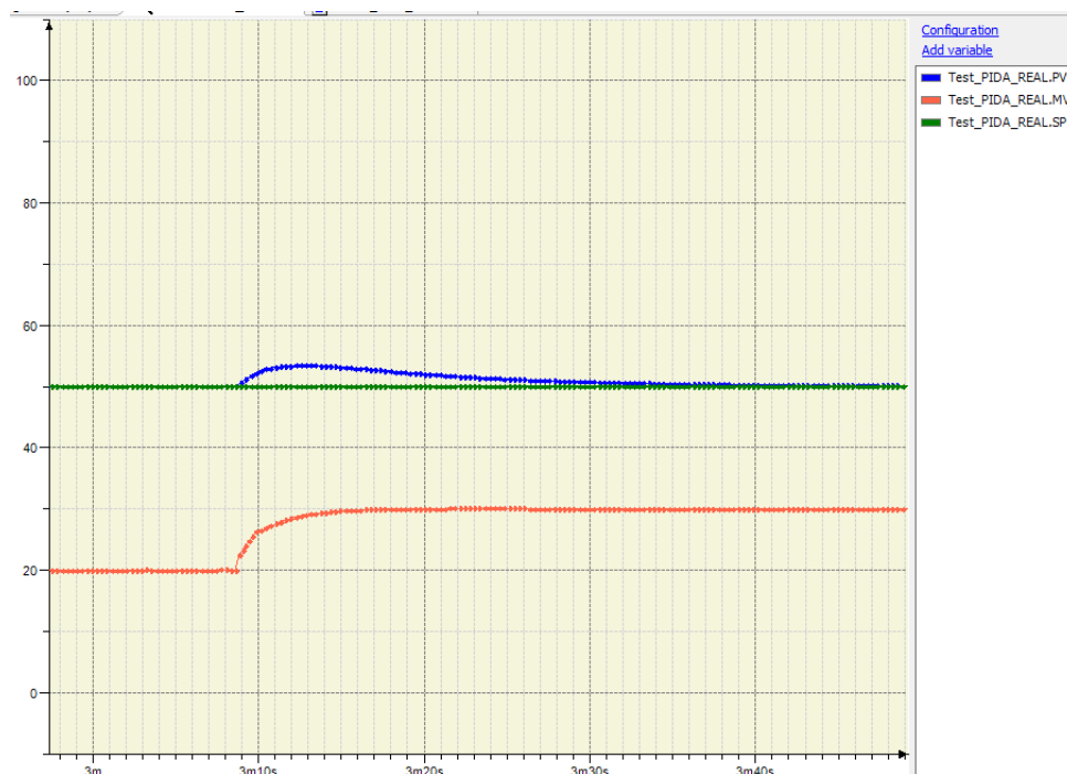
Figure 8: Example with direct control (Direct = TRUE)
