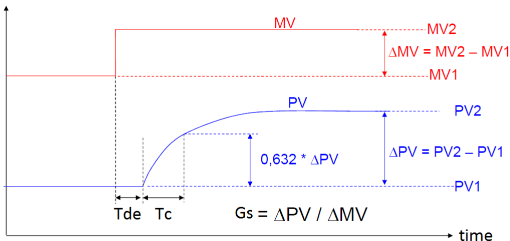
Figure 66: Open-loop process characterization
