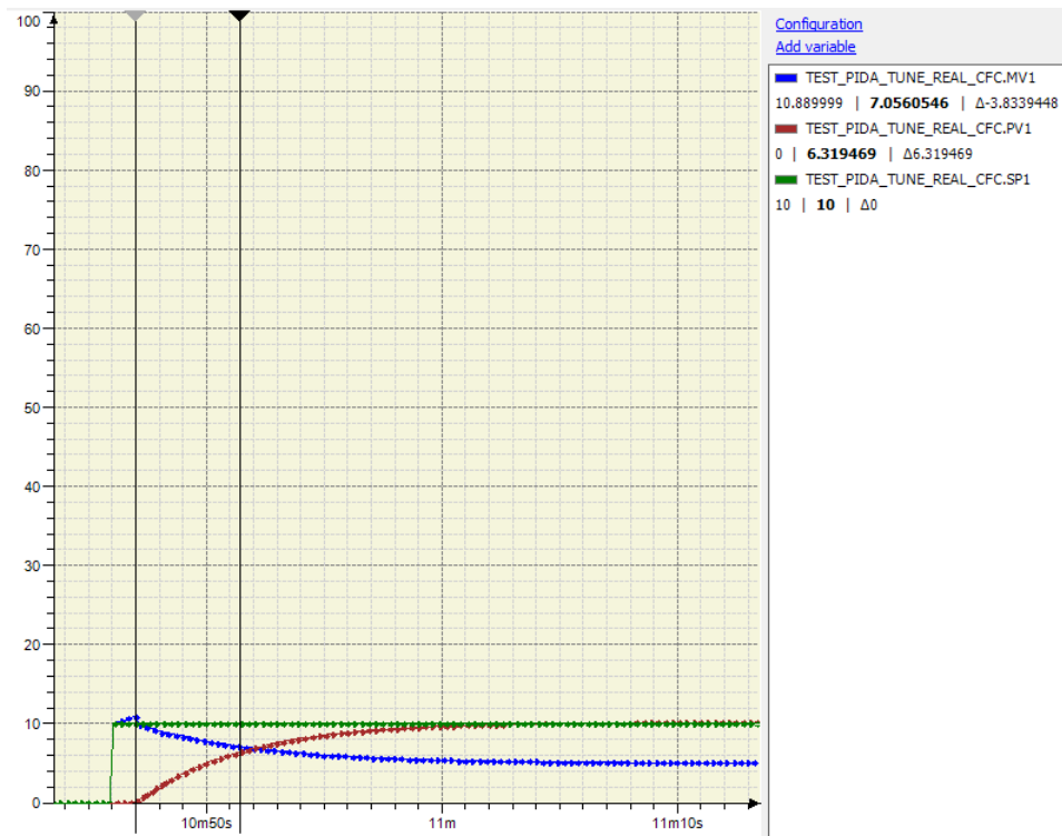
Figure 69: Automatic mode - closed loop time constant
