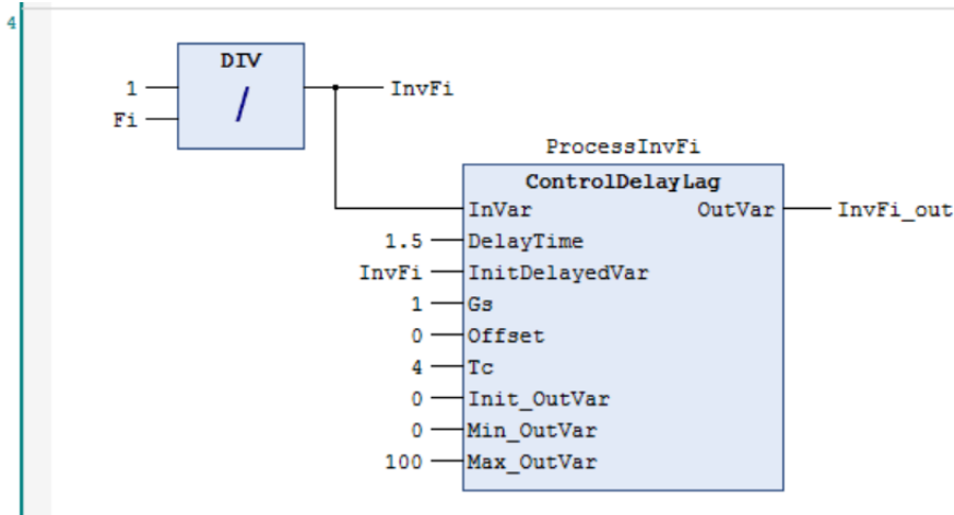
Figure 55: Network 4 of feed-forward example
