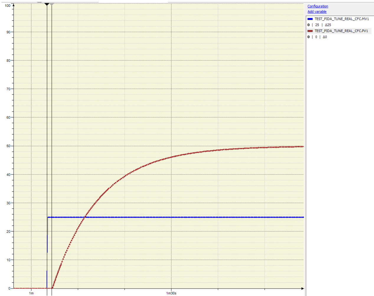
Figure 67: Open-loop characterization of process - dead time
