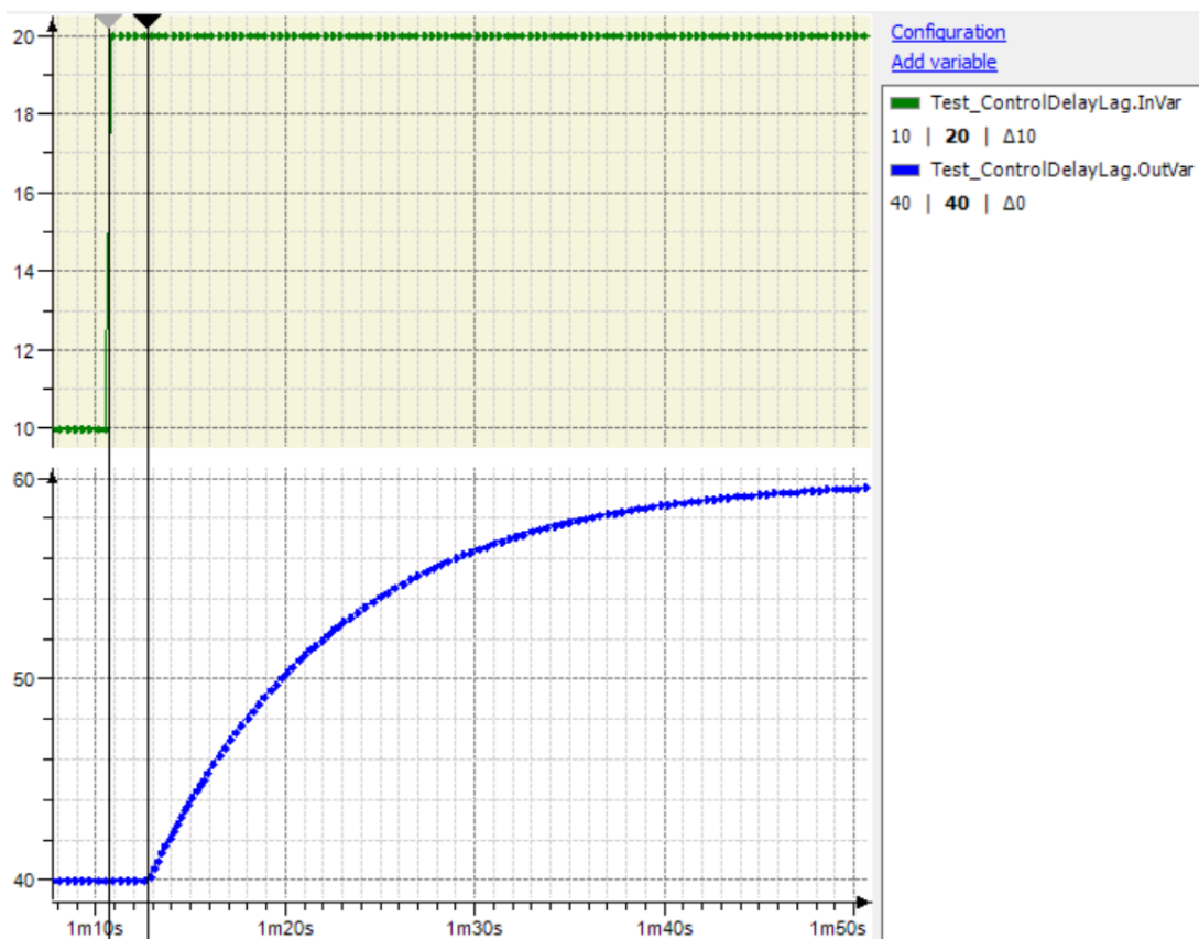
Figure 34: Example of delay plus lag created by ControlDelayLag
