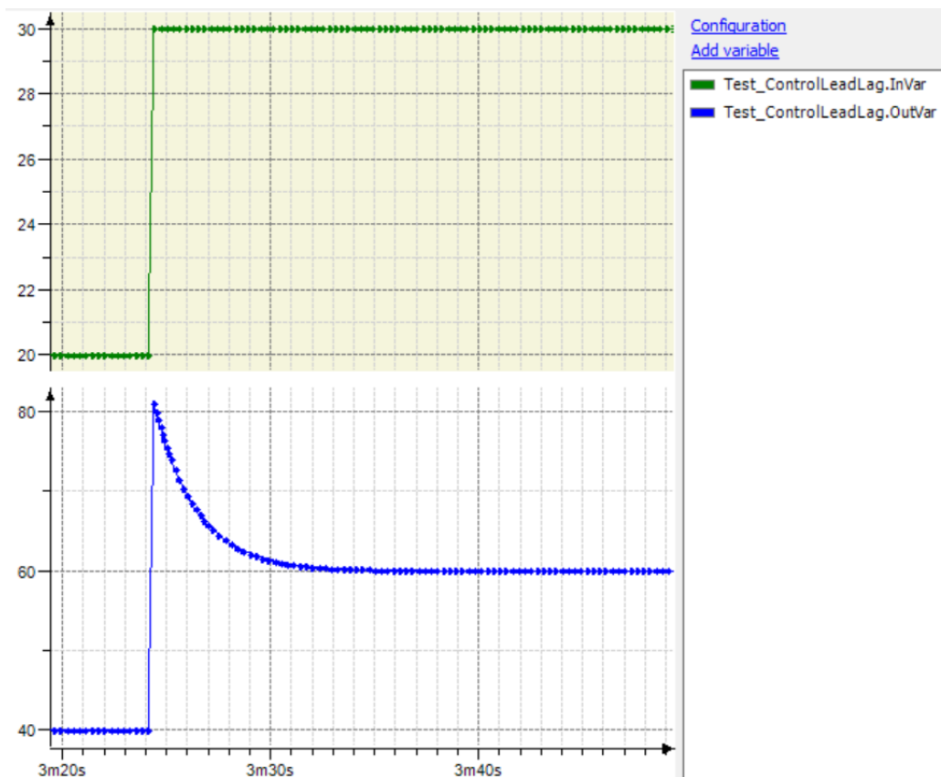
Figure 36: Example of ControlLeadLag with Tlead = 4s and Tlag = 2s
