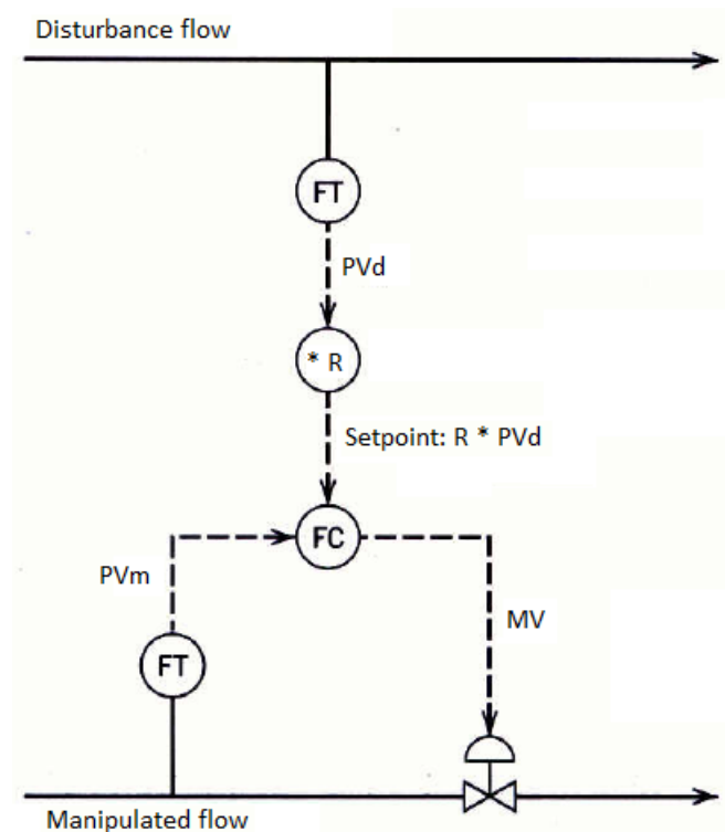
Figure 50: P&amp;ID for ratio control
