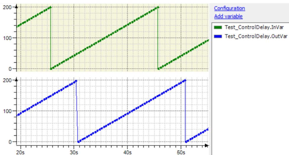
Figure 29: Example of delay created by ControlDelay
