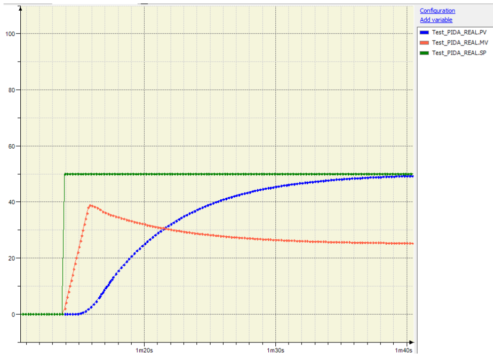
Figure 7: Response with MaxVarMV = 2 (with limitation, slower)
