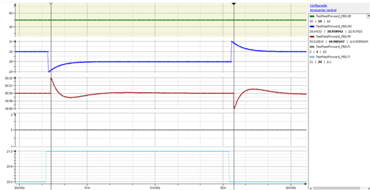
Figure 65: Effect of disturbances in T_i with feed-forward
