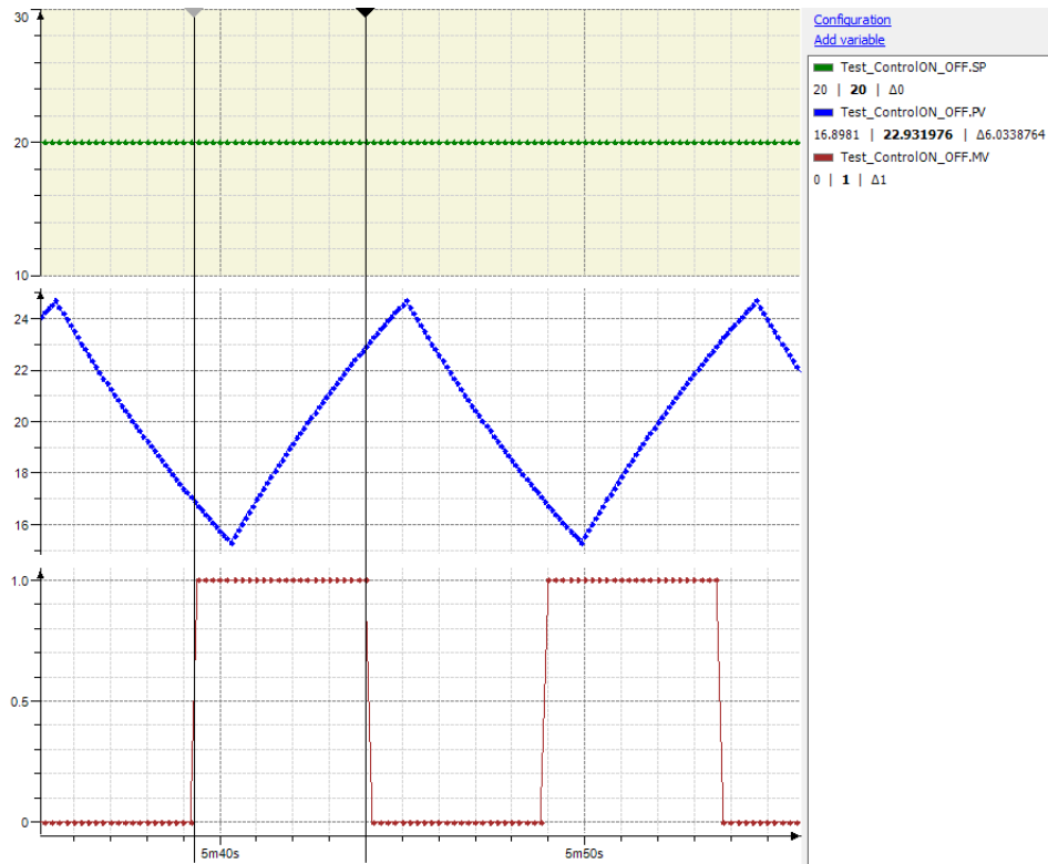
Figure 21: Example of ON OFF control
