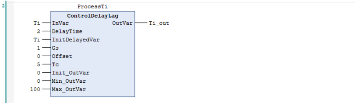
Figure 53: Network 2 of feed-forward example
