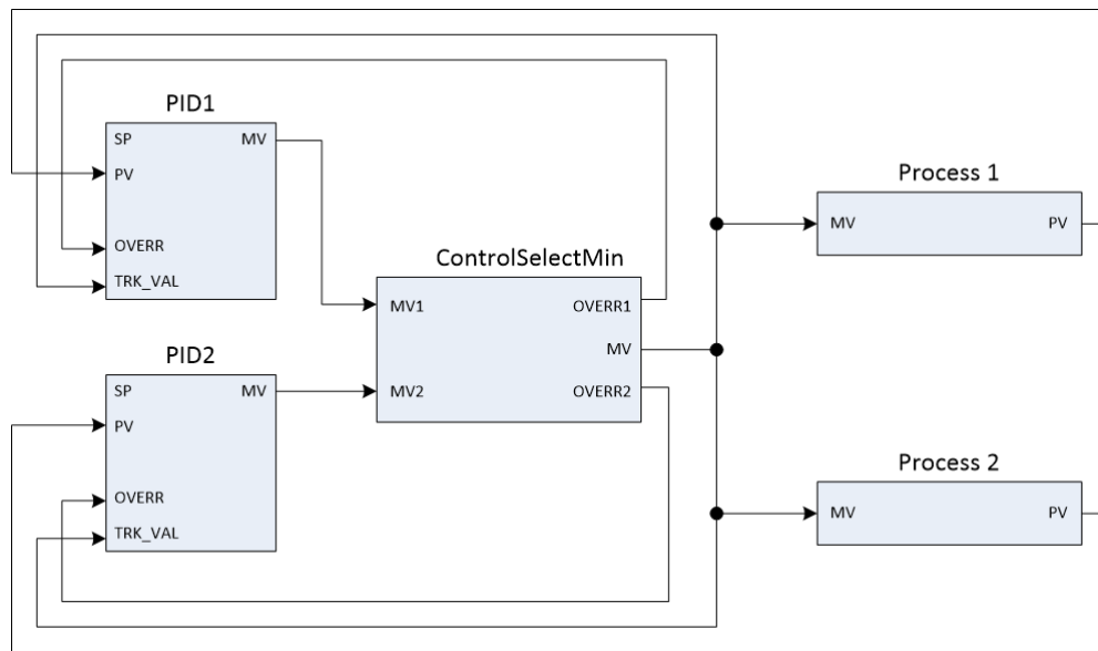
Figure 49: Special connections in override configuration
