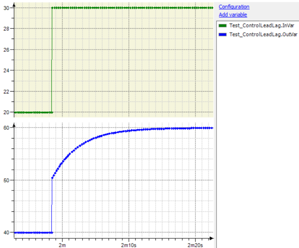
Figure 37: Example of ControlLeadLag with Tlead = 2s and Tlag = 4s
