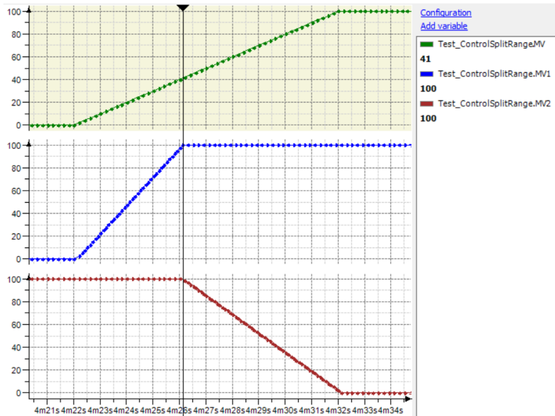
Figure 43: ControlSplitRange with Mode = 3 and SPLIT = 40%
