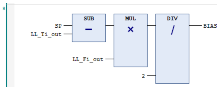
Figure 59: Network 8 of feed-forward example
