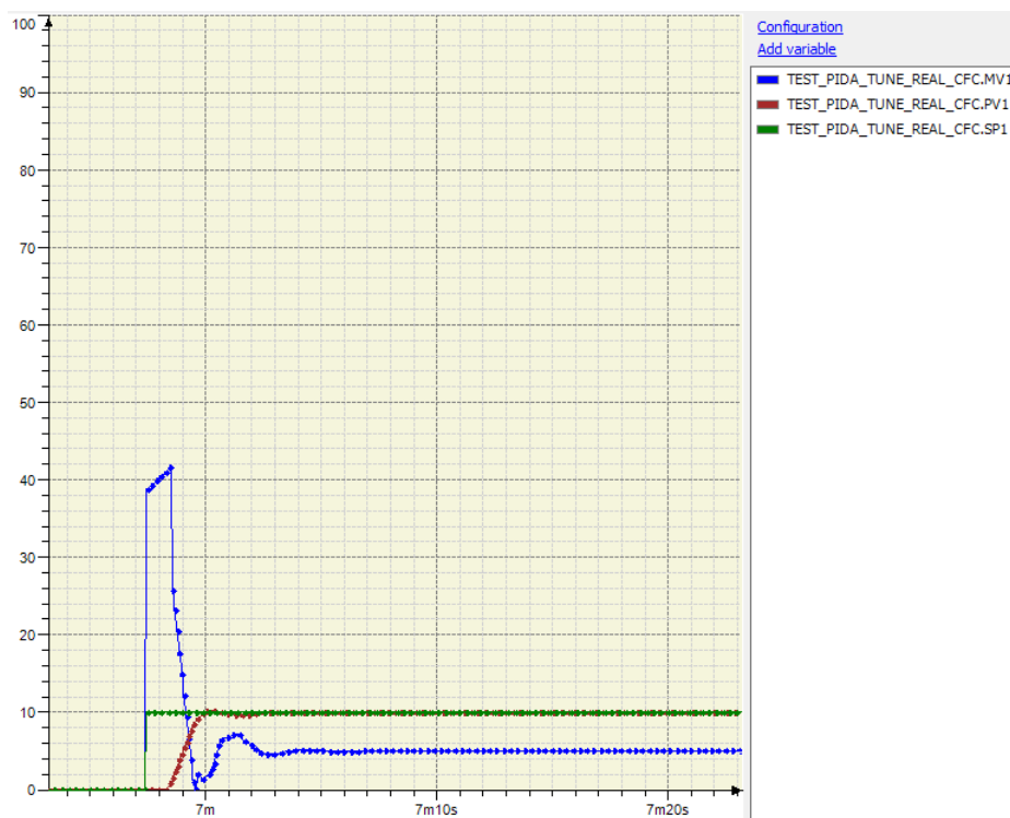
Figure 70: Tuning with minimization of integral of error for setpoint changes
