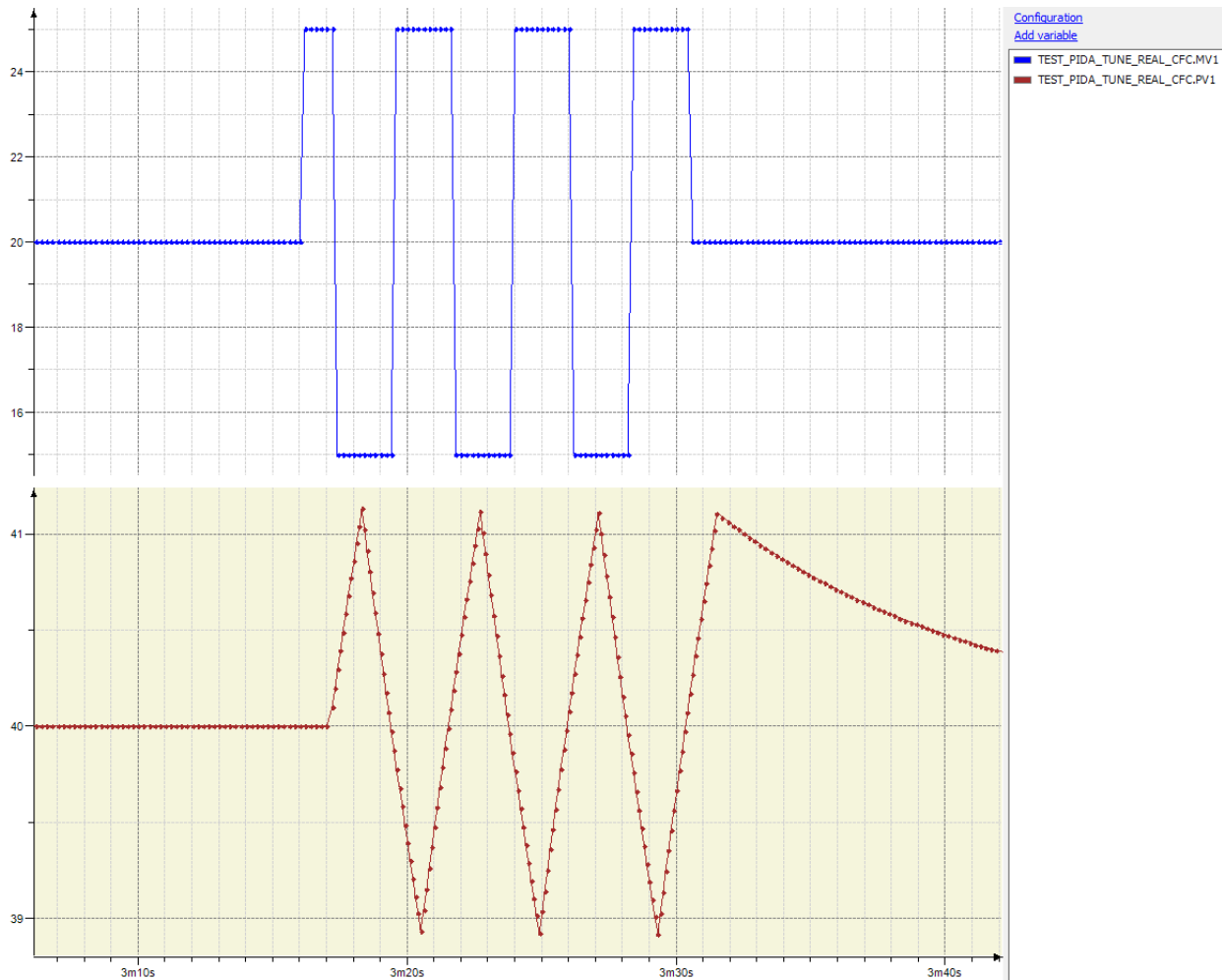
Figure 46: Example of PID simulation with auto-tuning
