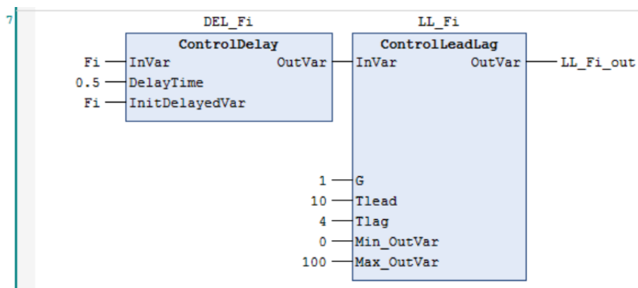
Figure 58: Network 7 of feed-forward example
