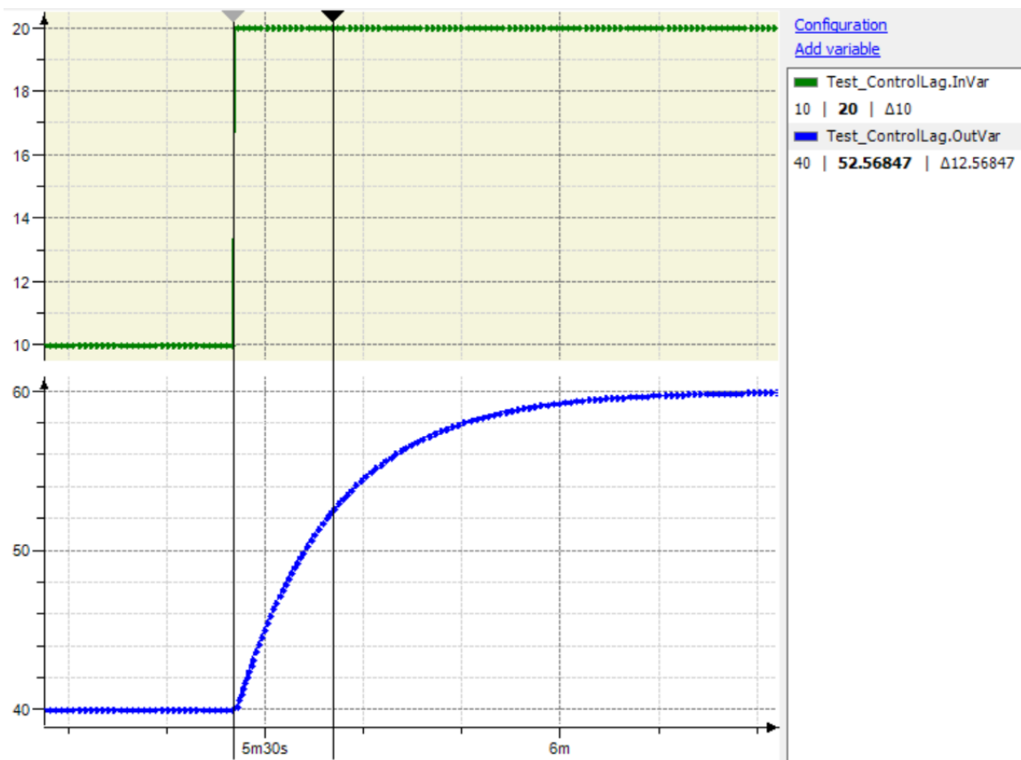
Figure 32: Example of lag created by Controllag
