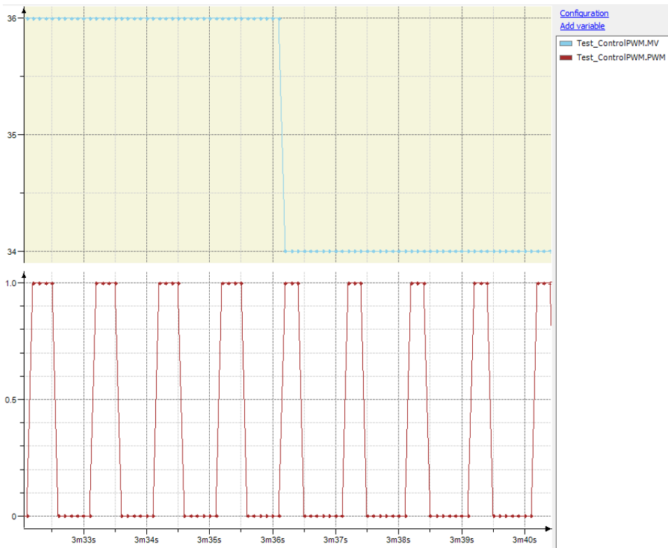
Figure 25: Example of ControlPWM conversion
