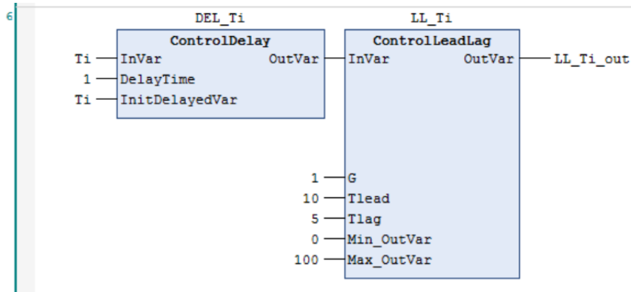
Figure 57: Network 6 of feed-forward example
