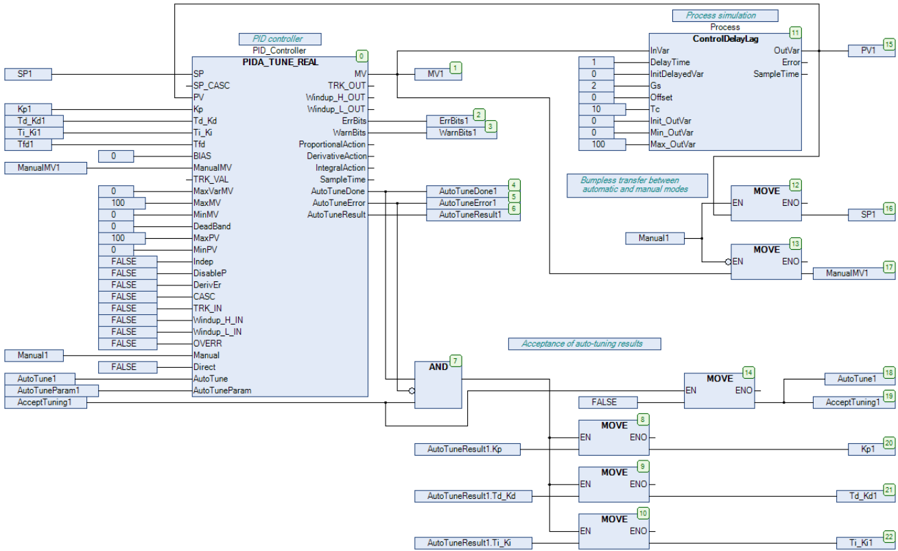
Figure 45: Example of PID simulation with auto-tuning
