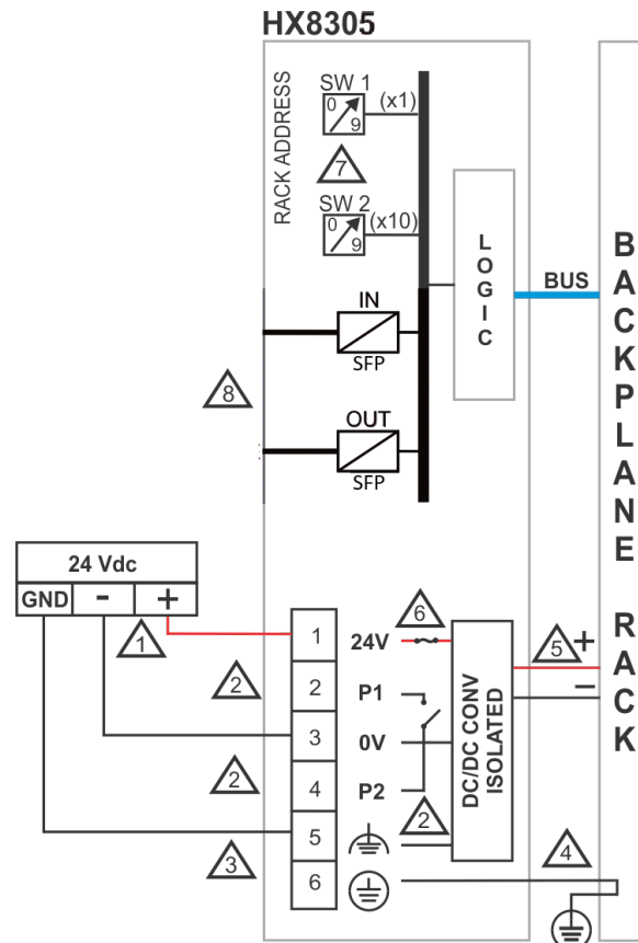
Figure 6: HX8305 Module Installation
