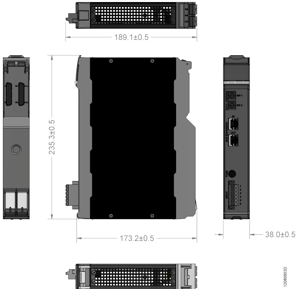
Figure 5: Physical Dimensions
