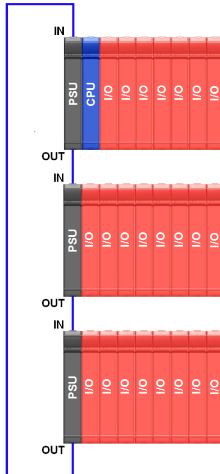
Figure 3: Bus Expansion with Loopback
