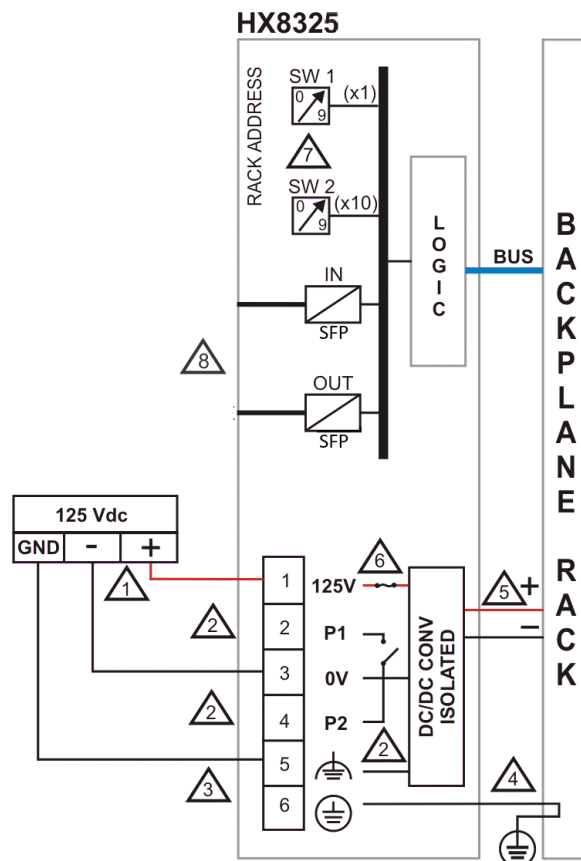
Figure 7: HX8325 Module Installation
