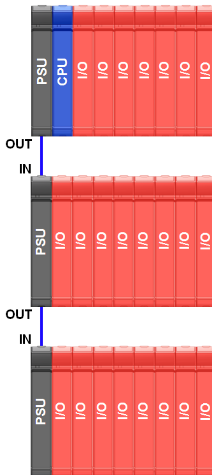
Figure 2: Bus Expansion without Loopback
